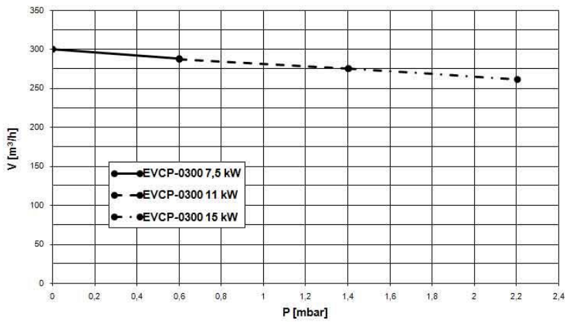
Capacity curve
