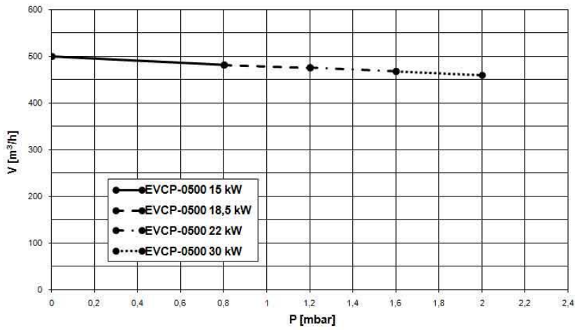
Capacity curve
