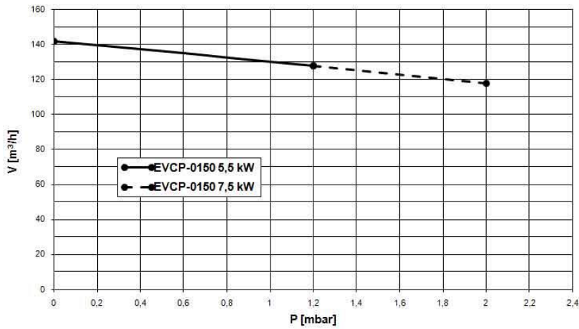
Capacity curve
