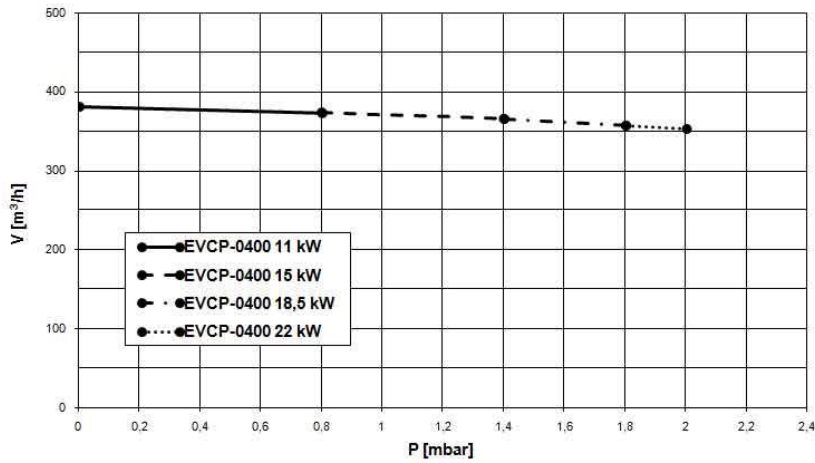
Capacity curve
