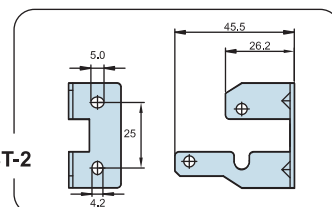
Panel adapter
