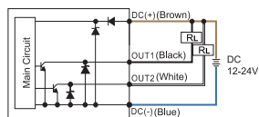
KP25□-02-□-□ NPN Output
