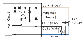
KP25□-04-□-□ PNP Output
